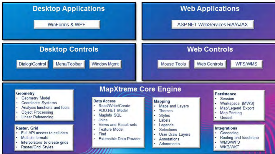
MapXtreme Architecture
